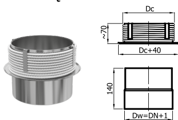
WKC
